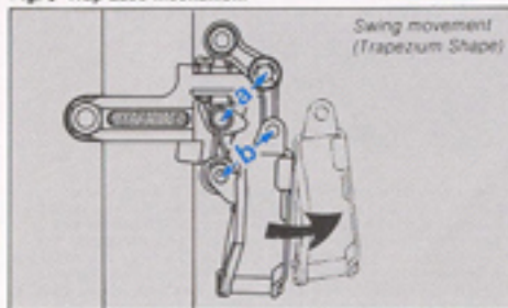
Fig. 6 Trap-Ease Mechanism
