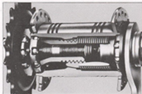
Sectional View of Coaster Brake
